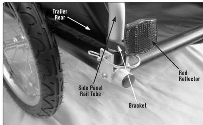
PHOTO 7: FLATBED RED REFLECTOR/BRACKET MOUNTED ON REAR CORNER OF SIDE PANEL RAIL TUBE
