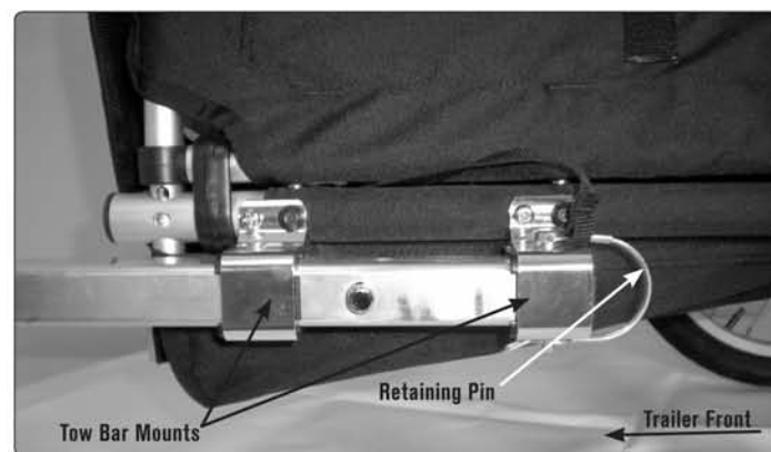
PHOTO 9: NOMAD TOW BAR INSTALLATION
